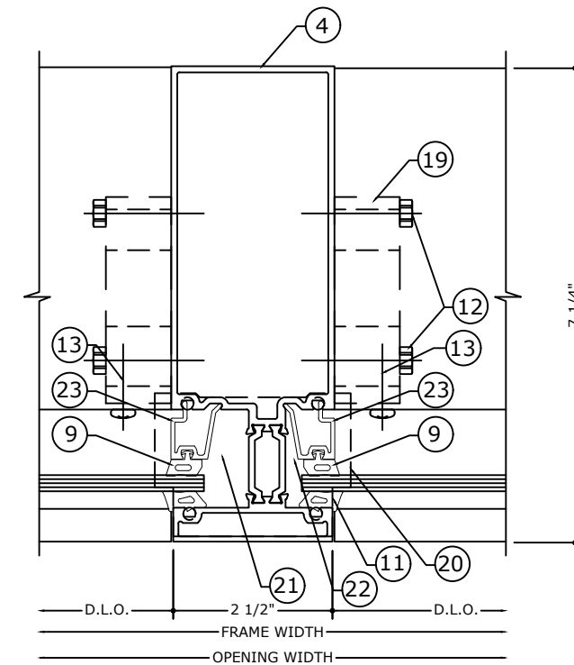
5.1 VERTICAL DETAIL - M1
