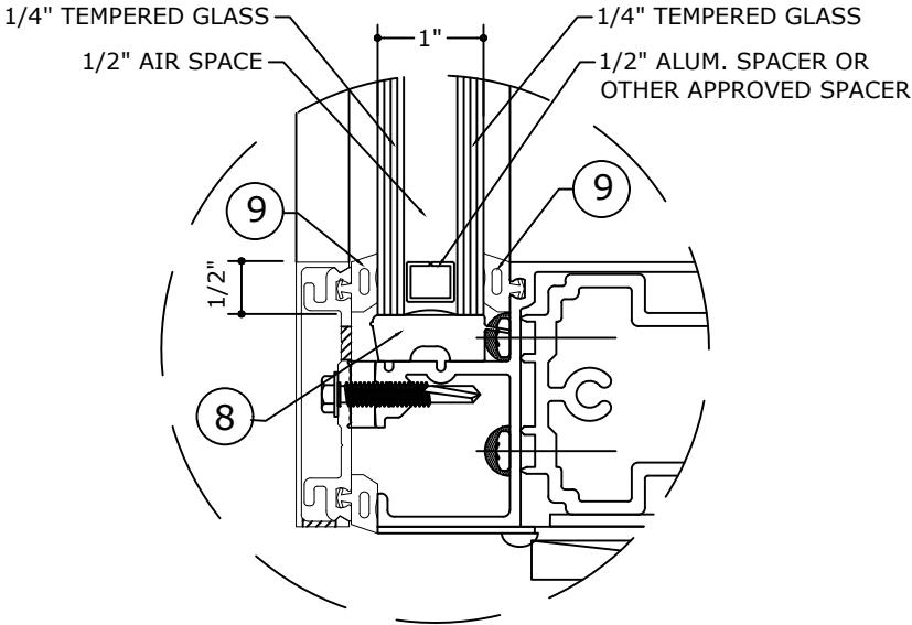
GLASS TYPE G1 GLAZING DETAIL N.T.S. GLASS RATING: NON IMPACT
