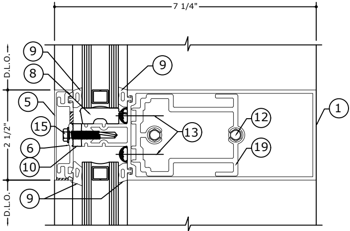
3 INTERMEDIATE HORIZONTAL DETAIL SCALE: 6" = 1'-0"
