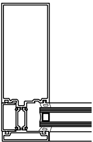
J1 DETAIL 4
