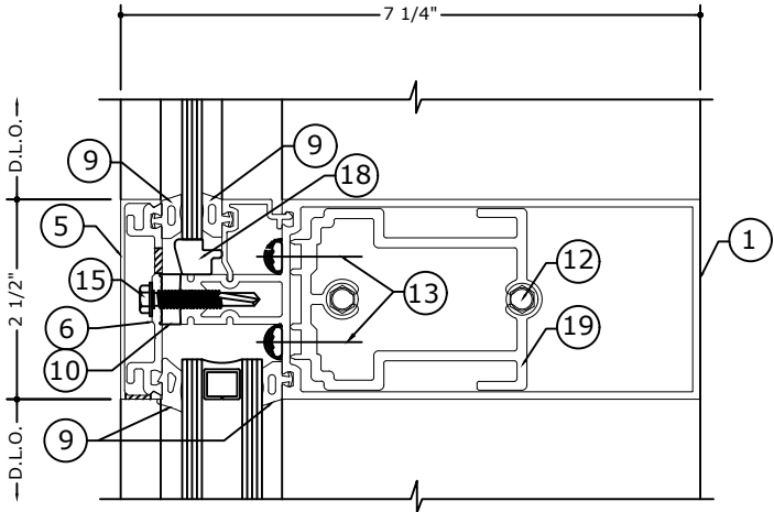
3.1 INTERMEDIATE HORIZONTAL DETAIL SCALE: 6" = 1'-0"
