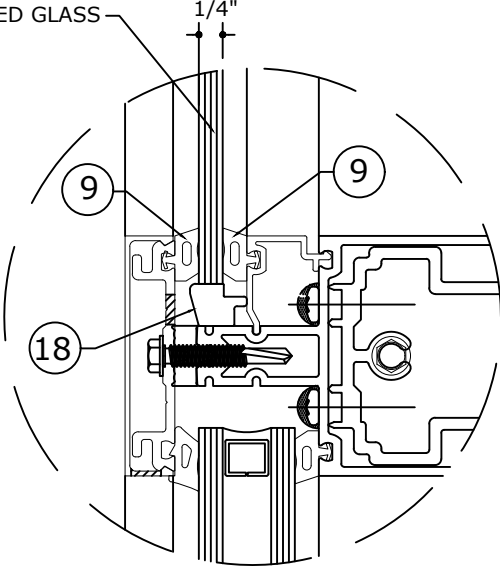
GLASS TYPE G2 GLAZING DETAIL N.T.S. GLASS RATING: NON IMPACT
