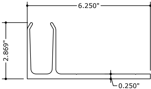
17 WW-103-05 "F" ANCHOR FOR WW-520
