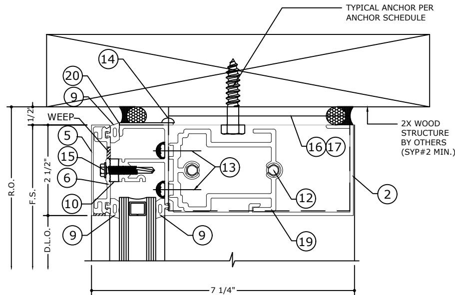
1.1 HEAD DETAIL
