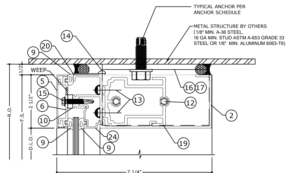
1.5 HEAD DETAIL
