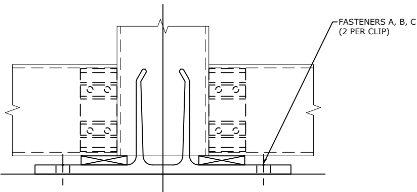
SILL DETAIL
