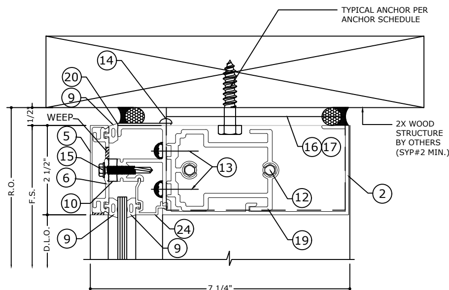
1.4 HEAD DETAIL
